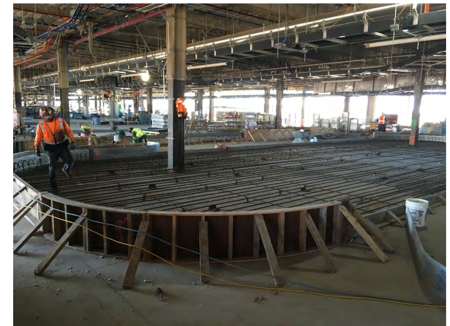
BHS Curb Formwork
